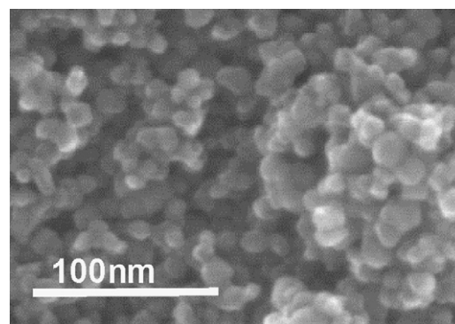
Fig. 6. SEM image of FP-6 (Showa Titanium; ca 15-nm primary particle size and 100 m 2 g -1 specific surface area).
