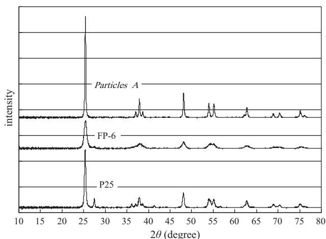
Fig. 5. XRD patterns of titania samples. Baselines were shifted for clarity.
