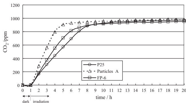
Fig. 4. Photocatalytic activity for mineralization of acetaldehyde in air.
