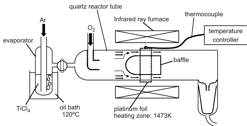
Fig. 1. Gas-phase reaction apparatus for the preparation of decahedral anatase titania particles.
