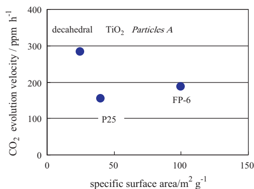
Fig. 7. Relationship between specific surface area and photocatalytic activity for mineralization of acetaldehyde in air.
