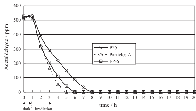
Fig. 4. Photocatalytic activity for mineralization of acetaldehyde in air.
