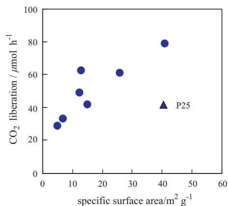
Fig. 3. Relationship between specific surface area and photocatalytic \text{CO}_2 production from an aqueous solution of 5 vol.% acetic acid. Circles: decahedral anatase titania particles. Triangle: P25.
