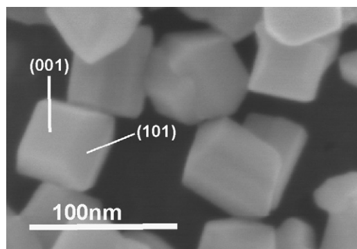
Fig. 2. SEM image of decahedral anatase titania particles prepared through gas-phase process. Particles A (ca 70-nm primary particle size and 25 \text{ m}^2 \text{ g}^{-1} specific surface area).
